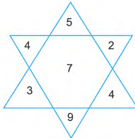
star B
