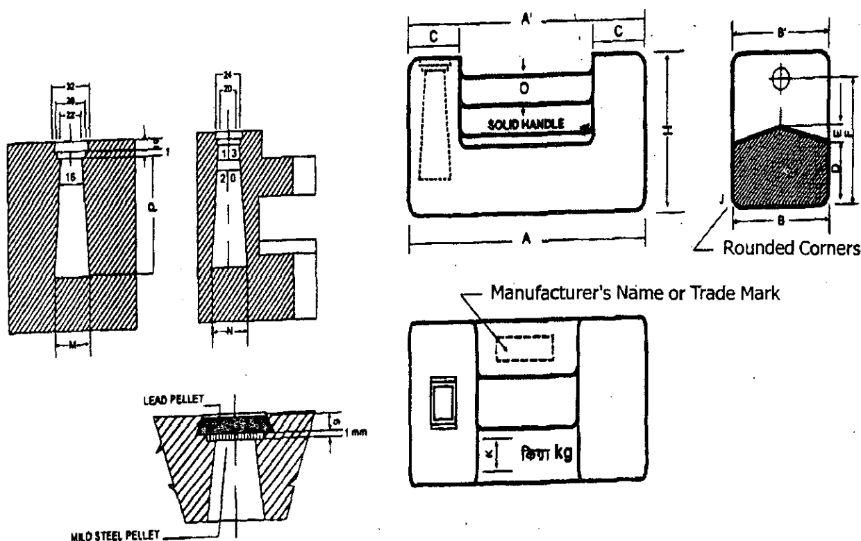
Parallelepiped Weight Type 2
